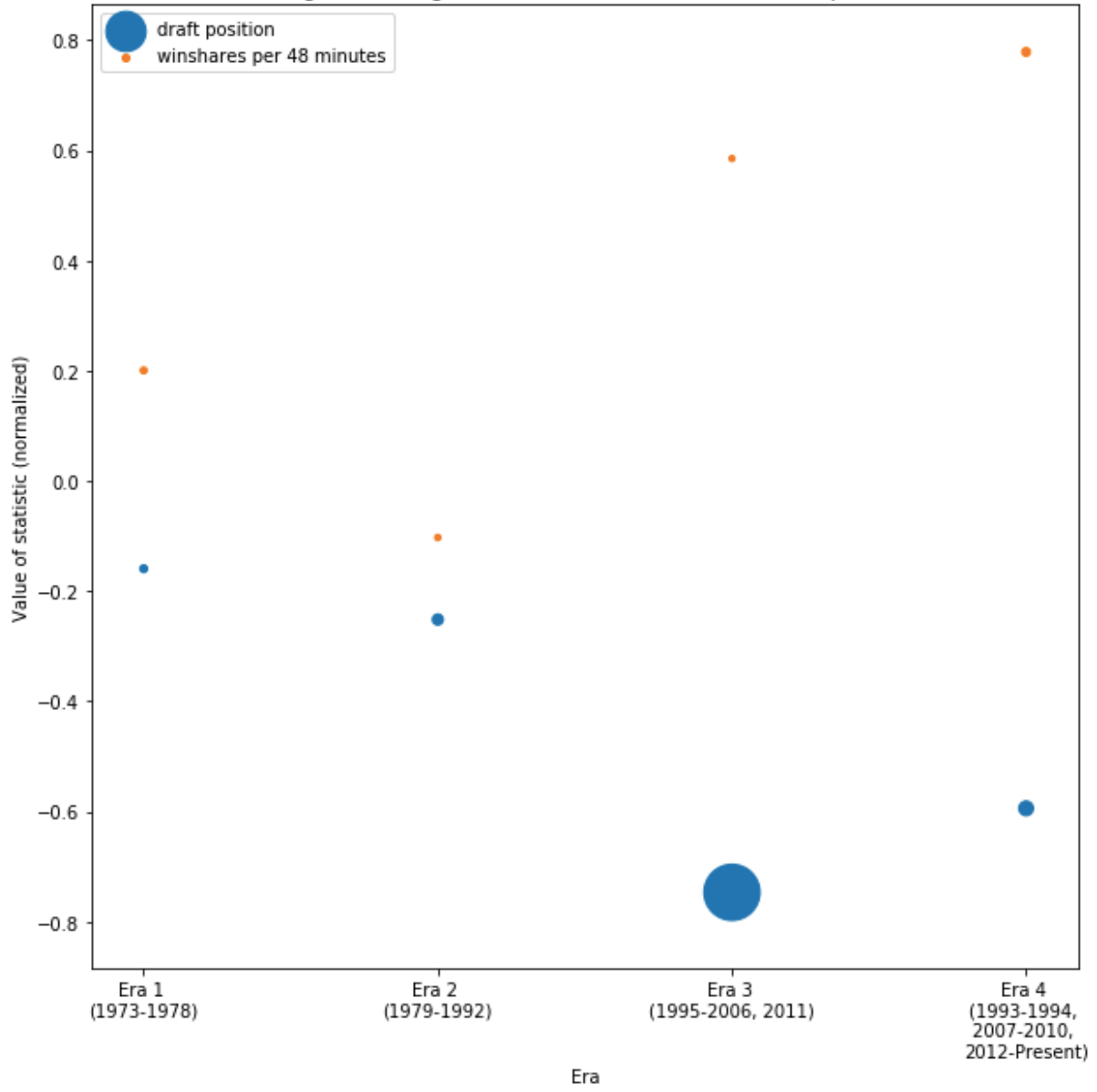
Weight for college winrate in Era vs Statistic, size=1/p-value
